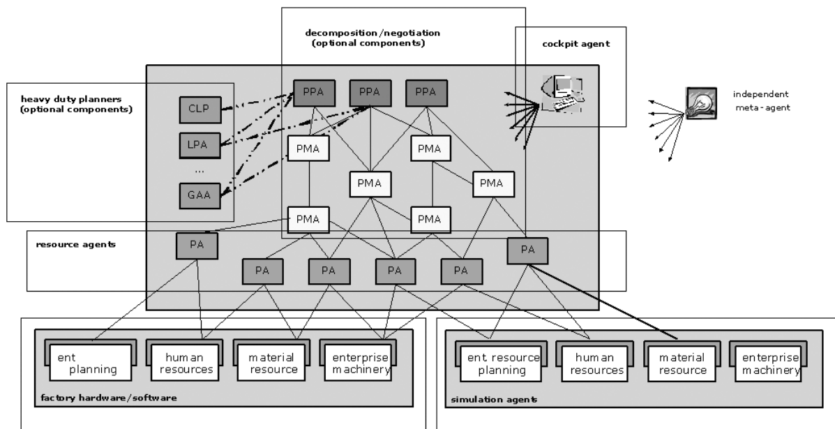
Figure 1 ExPlanTech Intra-Enterprise architecture
