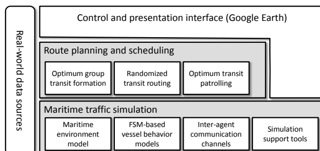
Figure 1: Architecture overview of the AGENTC system.
