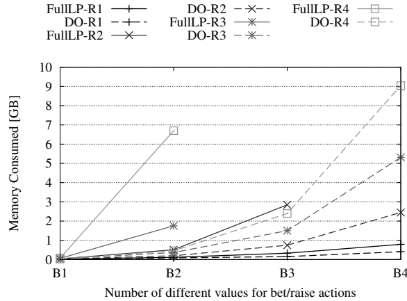
Figure 5: Memory consumption for instances of Poker games (R denotes number of re-raise actions, B number of possible betting amounts): solid lines represent FULLLP, dashed lines DO algorithm. Missing values for FULLLP indicate that the algorithm ran out of memory.
